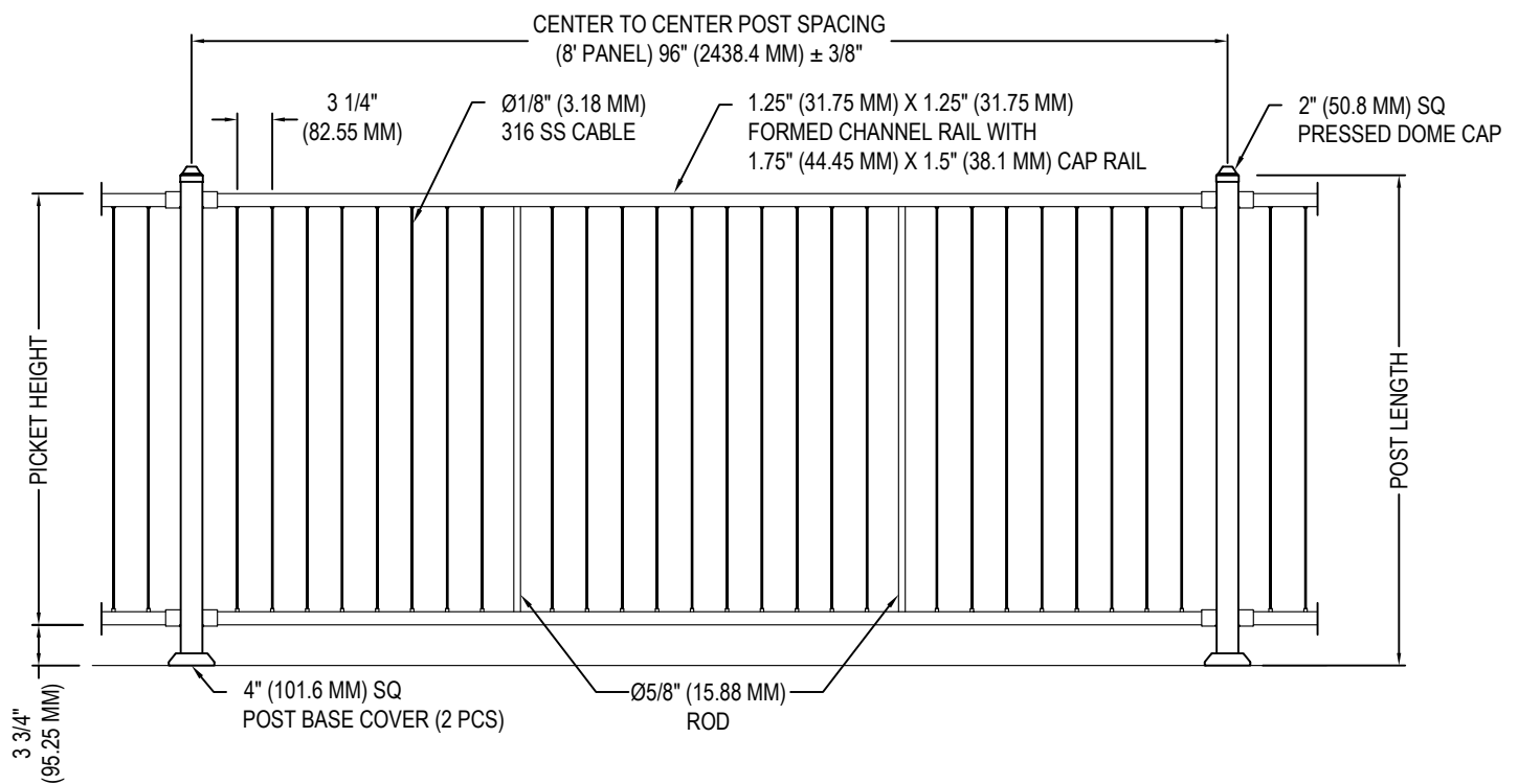
FRONT VIEW
